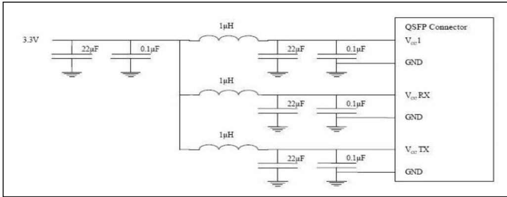
Host Board Power Supply Filtering
