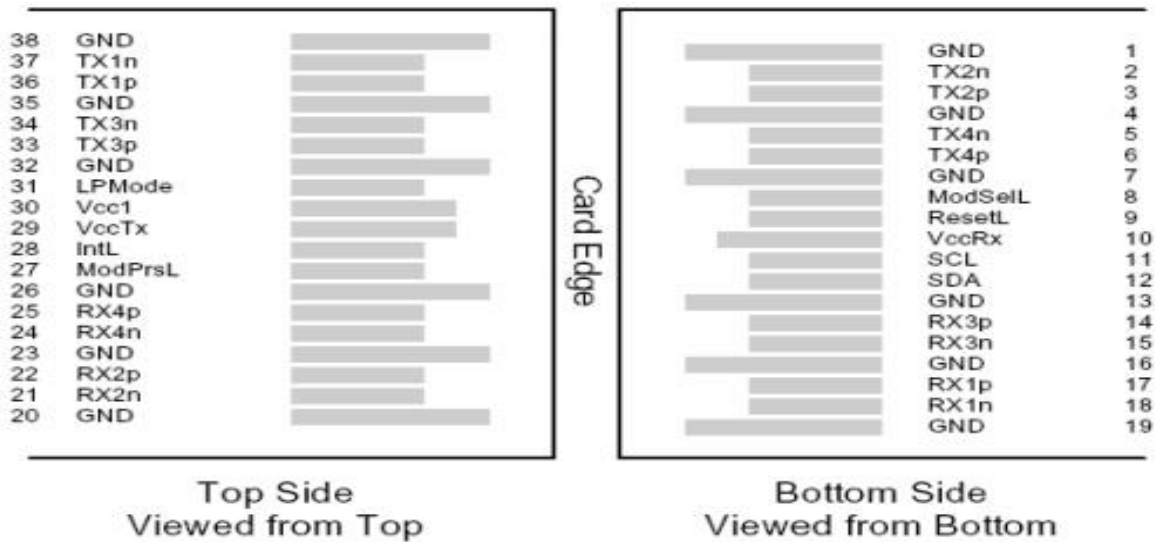
Figure 1 – QSFP+ MSA-compliant 38-pin connector
